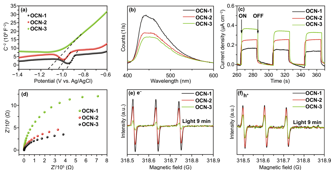
Fig. 4 a Mott–Schottky plots, b steady-state photoluminescence (PL) spectra, c transient photocurrent responses, d EIS spectroscopies, e , f ESR spectra of e^- and h^+ of OCN-1, OCN-2, and OCN-3 under visible-light irradiation for 9 min
