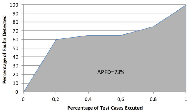
Fig. 6 APFD of local beam search for an arbitrary test suite
