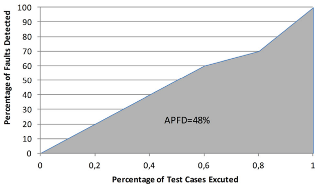
Fig. 5 APFD of greedy algorithm for an arbitrary test suite
