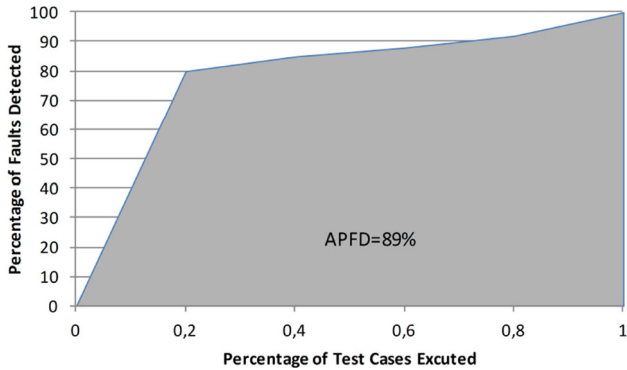
Fig. 7 APFD of BITCP algorithm for an arbitrary test suite
