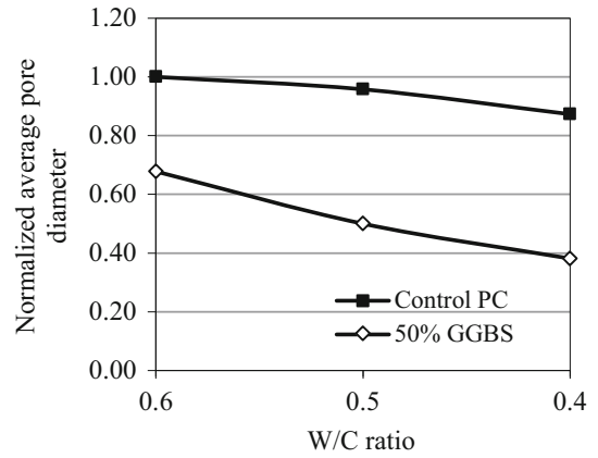
Fig. 5 Effect of w/c ratio on average pore diameter of concrete (at 28 days curing).
