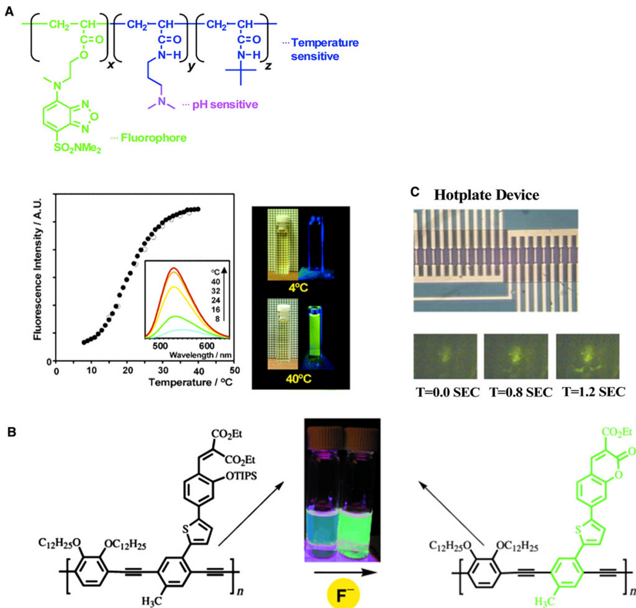
Fig. 6 A Fluorescent polymer sensor for temperature [186]. B Fluorescent polymer sensor for the detection of fluoride ions [194]. C Micrograph showing the microfluidic hot plate with gold hot lines
