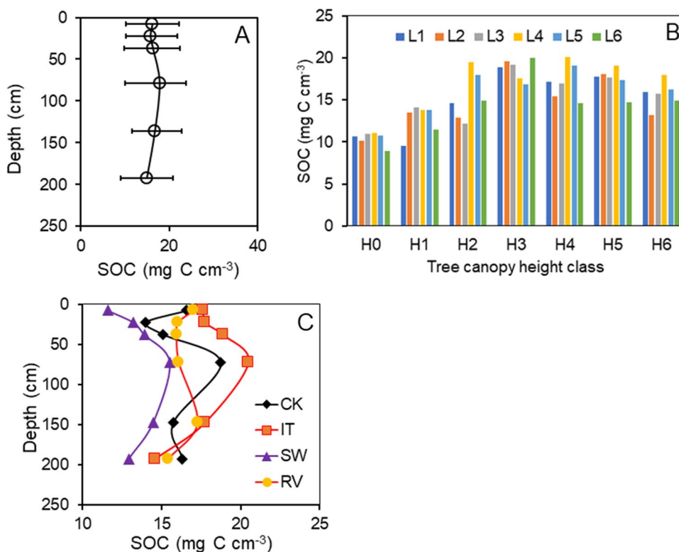
Fig. 4 Mean SOC (mg C cm -3 ) at different soil depths for mangrove soils (A), bars represent the standard deviation ( \pm 1 SD); means at different tree canopy height (B), sampling depth, L1: 0 – 15 cm, L2: 15 – 30 cm, L3: 30 – 45 cm, L4: 45 – 110 cm, L5: 110 – 185, L6: 185 – 200 cm; means in different hydrogeomorphic settings (C); CK: Creek; IT: Interior; RV: Riverine; SW: Seaward
