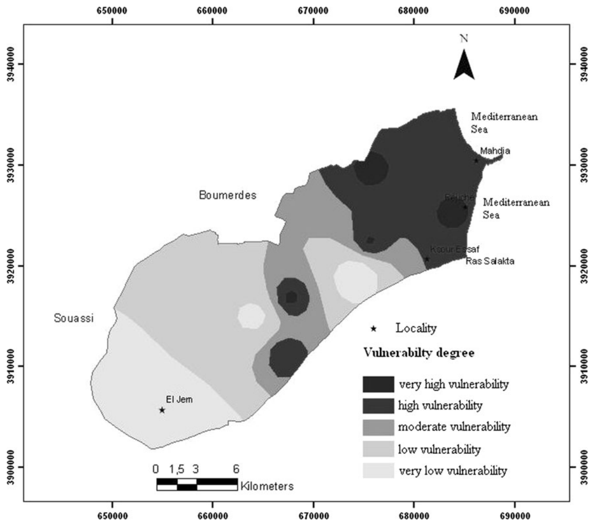
Fig. 7 Groundwater vulnerability of the Mahdia–Ksour Essaf aquifer using AVI method (Saidi 2011)
