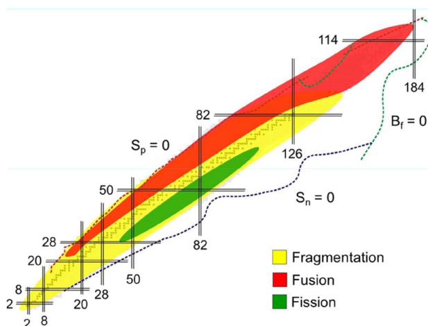
Fig. 2 Chart of the nuclides with indication of the main mechanisms for production of artificial isotopes. Fragmentation reactions produce both neutron-rich and neutron-deficient nuclei up to uranium (yellow area). Fission reactions lead to relatively neutron-rich, intermediate heavy nuclei (green area). Fusion reactions enable to synthesize transuranium and superheavy nuclei, but rather in the neutron-deficient region with respect to the stability line (red area) (Reproduced with permission from Adamian et al. 2020a, page 2) (Color figure online)
