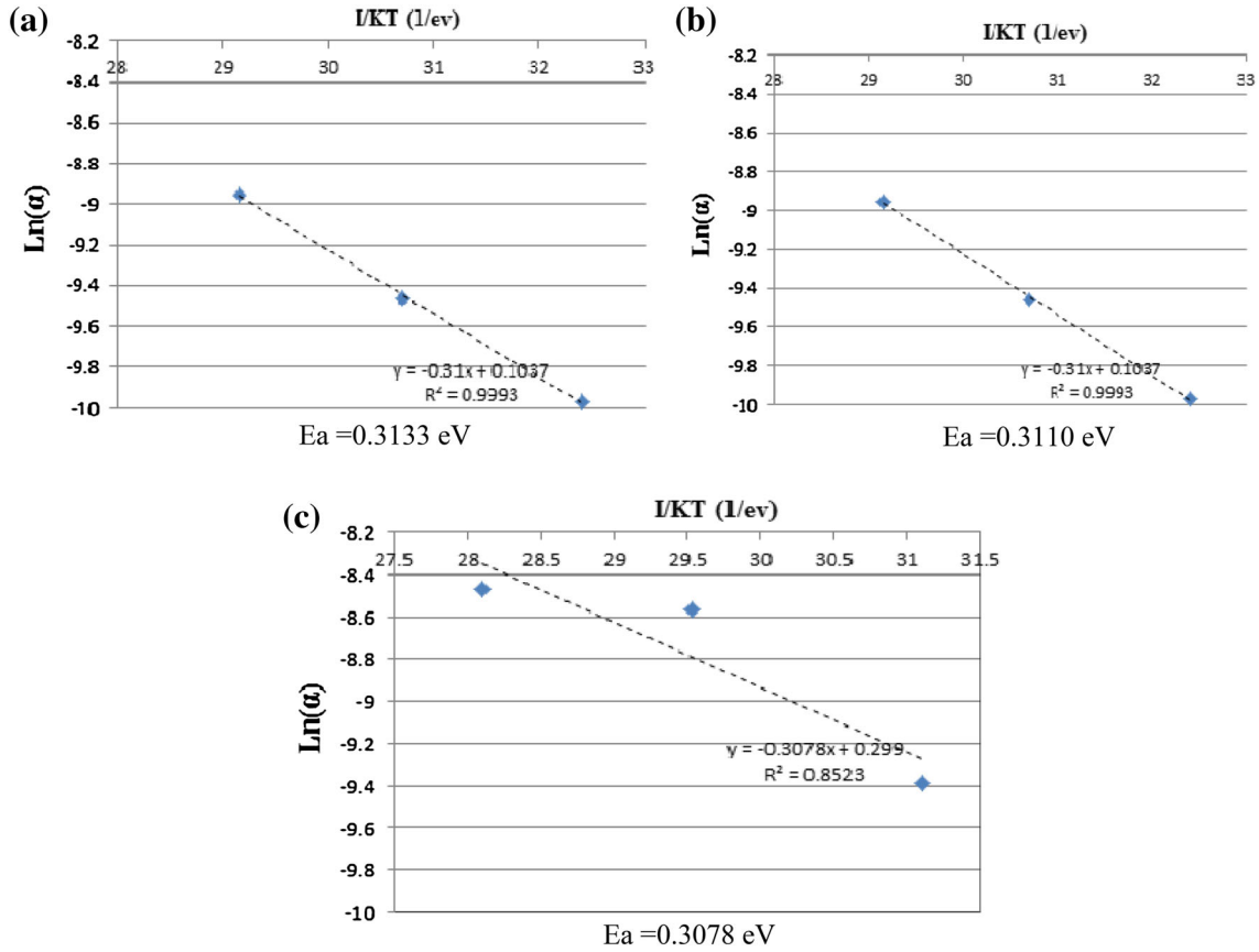
Fig. 4. Plot of \ln(\alpha) versus E/KT for remote phosphor (a) 825 \text{ W/m}^2 , (b) 3300 \text{ W/m}^2 and (c) 13,200 \text{ W/m}^2 .
