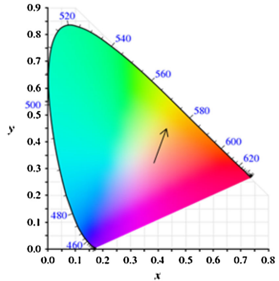
Fig. 5. The variation of chromatic chromaticity for 13,200 \text{ W/m}^2 at 120^\circ\text{C} .
