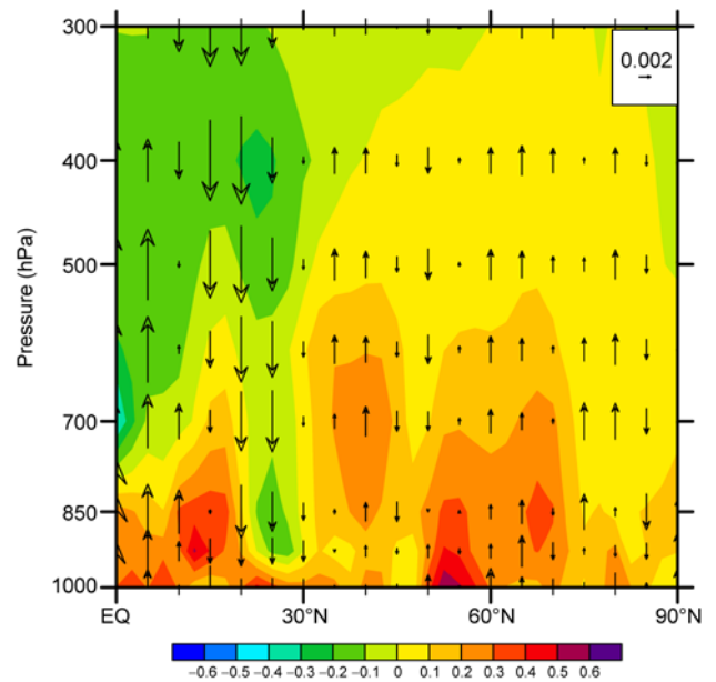
Figure 4 Meridional-vertical cross sections of interdecadal difference (Phase II minus Phase I) in vertical wind (Pa/s) and specific humidity ( \text{g}/\text{kg} ), averaged over 110^{\circ}\text{--}120^{\circ}\text{E} .
