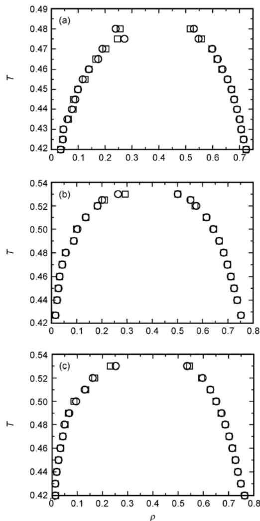
Figure 2 Gas-liquid phase coexistence using different interaction truncations. The number of particles is N=256 . r_{\text{cut}}=2.5 (a), 5.0 (b), L/2 (c). Note that the long-range correction is only applied for r_{\text{cut}}=L/2 . Open circles (squares) represent results obtained under compression (expansion).
