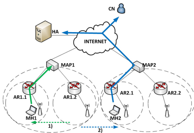
Fig. 4 Hierarchical Mobile IPv6 scenarios 1 Micro-mobility handover (in the scope of the same MAP), Local Binding Update proceed to MAP, 2 Macro-mobility handover, Home Binding Update proceed to HA and CN
