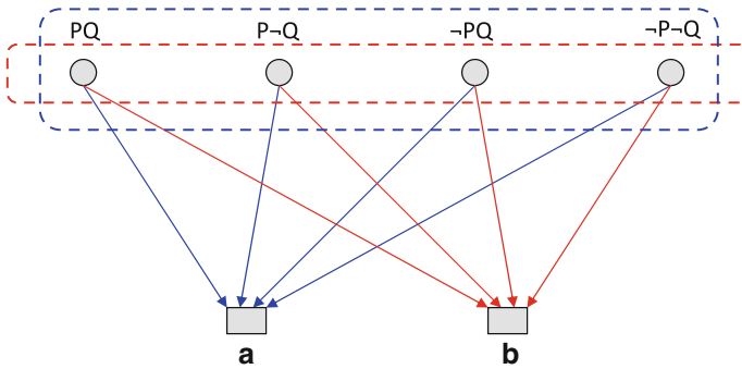
Fig. 4 The failure of measurability
