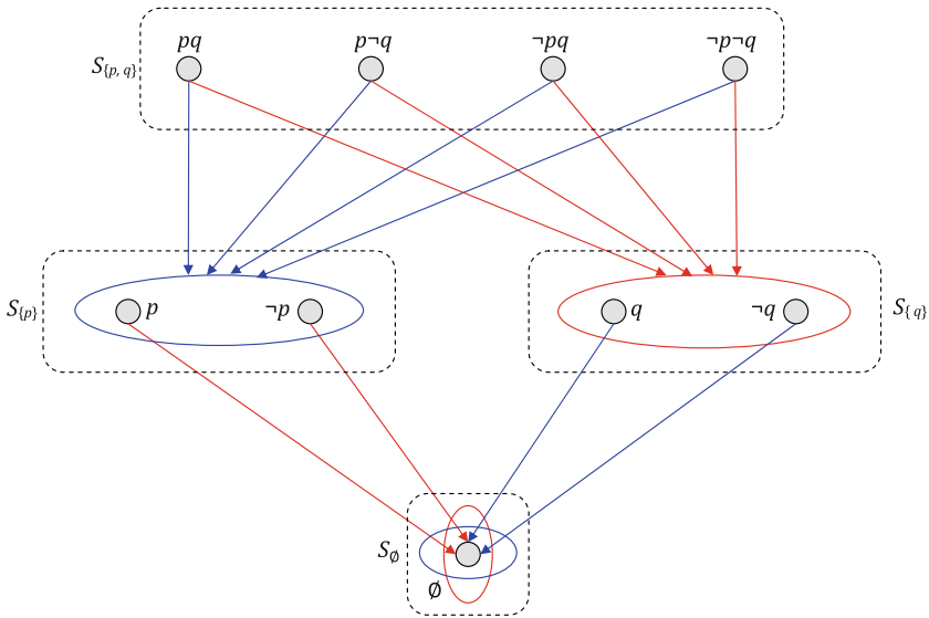
Fig. 3 The failure of KU -Introspection
