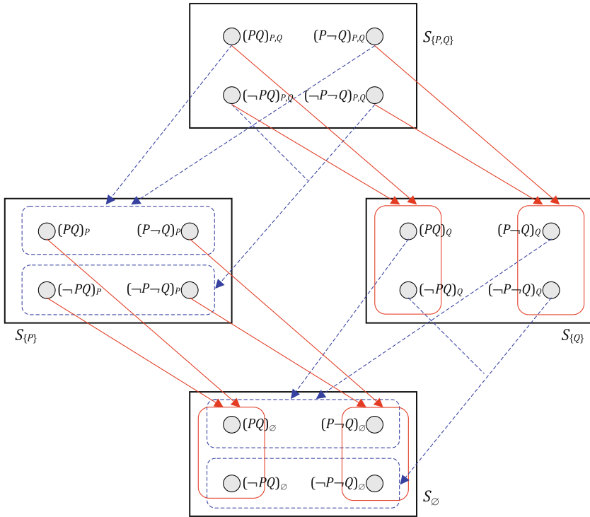
Fig. 2 Example of an HMS structure
