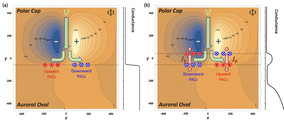
Fig. 4 From Ohtani et al. (2018): Schematic explanation of the deflection of the fast polar cap flow (light green arrow coming from the top) at (a) the step-like change of the ionospheric conduction and (b) the band of the enhanced conduction (as illustrated to the right of each panel). The electrostatic potential is shown by contours and colors, which was adopted from Fig. 5e of Ohtani and Yoshikawa (2016); although their model calculation was conducted for a step-like change of conduction, we adopted it here for both panels. The contours are squeezed out of the auroral oval (bottom half) to the polar cap (top half) because of electrostatic polarization at the poleward boundary. The vertically elongated area of dense potential contours in the middle of the polar cap corresponds to the flow channel. In panel (b) the intensities of the ionospheric Pedersen currents ( J_p ) inside and outside of the conduction band are schematically shown by the arrows in magenta. See Ohtani and Yoshikawa (2016) for more details
