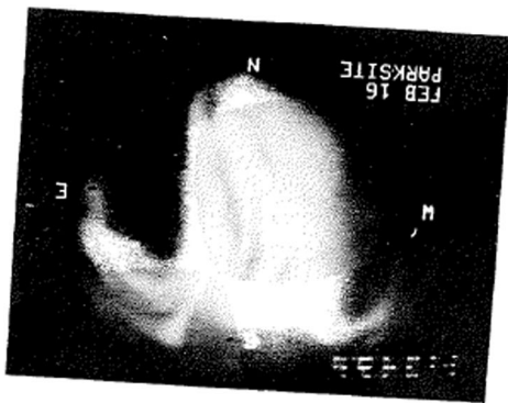
Fig. 10 An auroral torch is an activity center for pulsating aurora. (Adapted from Oguti 1981)
