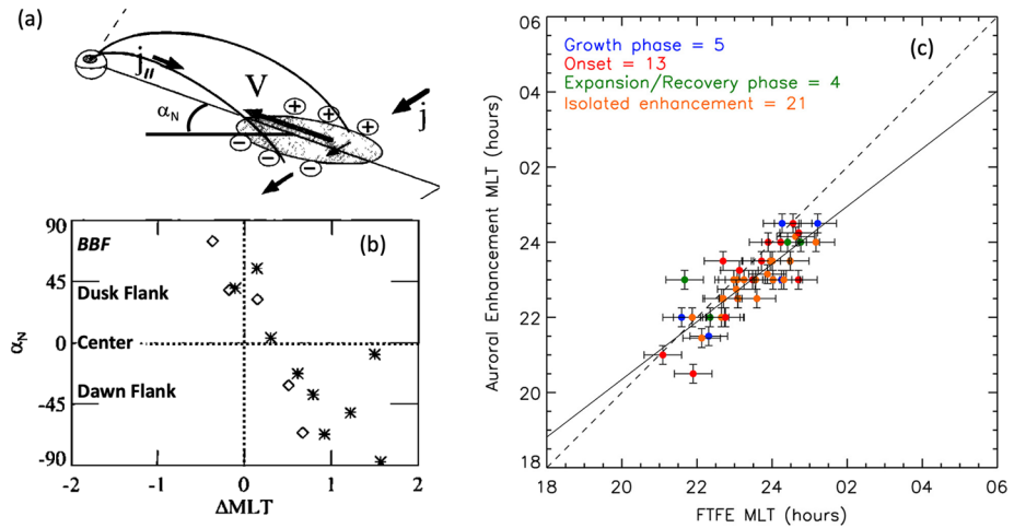
Fig. 8 (a) Scheme of fast flow channel (BBF), and, (b) – relationship of MLT difference between BBF ionospheric footprint and streamer ( \Delta MLT = MLT_{\text{msph}} - MLT_{\text{isph}} ) against the angle \alpha_N characterizing which BBF side was crossed by spacecraft (both after Nakamura et al. 2001). Diamonds (or crosses) indicate the streamers (or localized brightenings) observed in the ionosphere. (c) MLT comparison of fast tailward flows (FTFE) footprint and auroral brightenings from Case et al. (2017); red ellipse helps to see that \sim 1 h MLT-wide points cloud lay under the diagonal (shown by dashed black line) indicating a systematic dawnward shift of FTFE footprints from their related optical effects. See text for discussion
