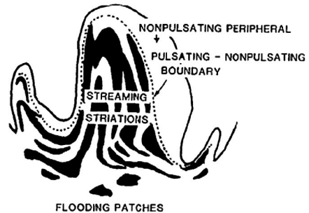
Fig. 10 An auroral torch is an activity center for pulsating aurora. (Adapted from Oguti 1981)
