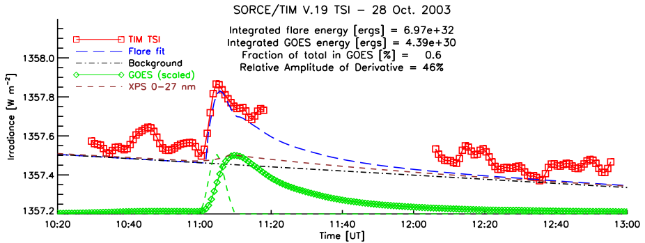
Figure 11 The X17 flare on 28 October 2003 was the first ever observed in TSI (red squares). A fit (dashed blue line) including a linearly varying background (dot-dashed black line) is based on GOES data (green diamonds) and its derivative (dashed green line), which is representative of the impulsive phase of the flare. [Updated data version and plot from that in Woods, Kopp, and Chamberlin, 2006.]
