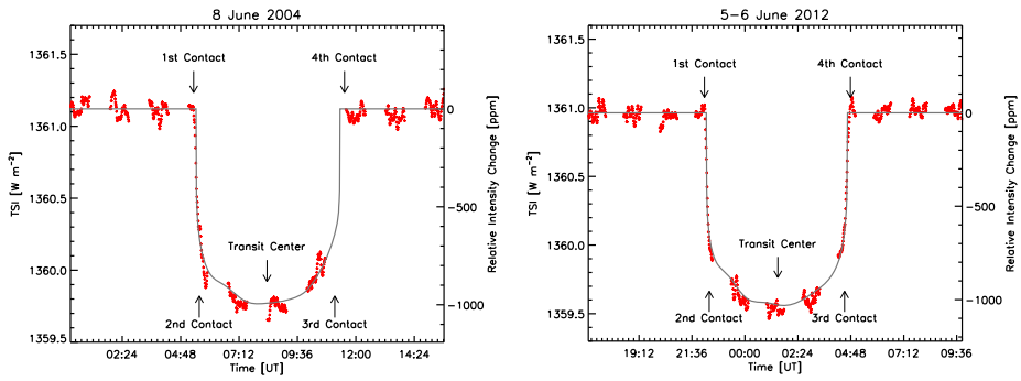
Figure 12 The SORCE /TIM observed two Venus transits across the solar disk. The red dots are the TSI measurements, which closely match the predicted transit light curve (gray line) accounting for solar limb darkening and the SORCE position. The gaps in the plotted data are from times when the SORCE spacecraft was eclipsed by the Earth. The small fluctuations in brightness on short timescales are from normal solar convection and oscillations and can be seen in the un-occulted times both before and after the transits. All data are from SORCE /TIM V.19.
