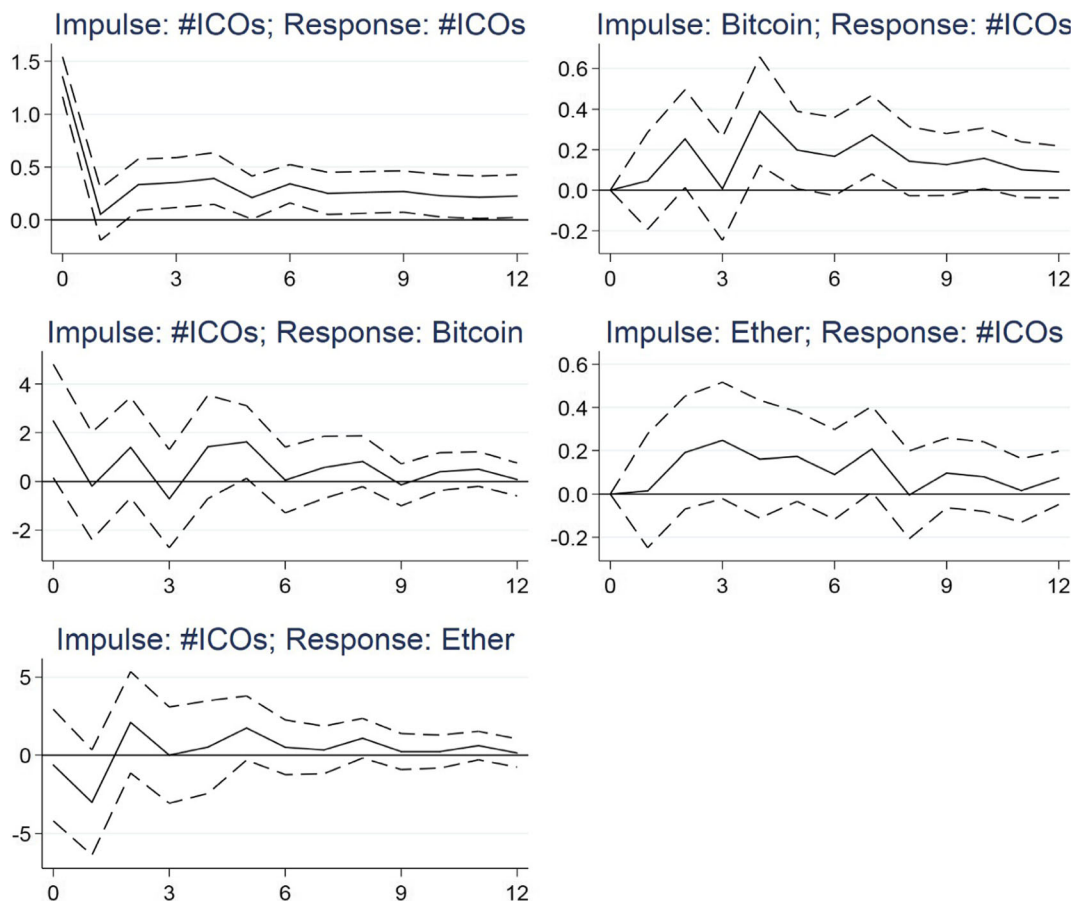
Fig. 8 Impulse responses of VAR model with number of ICOs. The figure shows the impulse responses (solid lines, in percentage points) to a one standard deviation shock in the ICO growth rates (left panel), bitcoin returns (upper right figure), and ether returns
