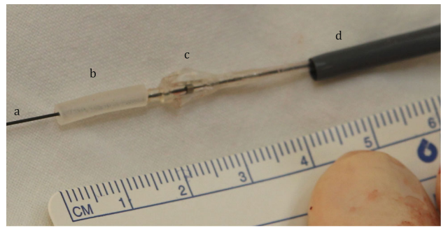
Fig. 1 Delivery device with guidewire (a), hydrogel (b), occlusion balloon (c), and delivery sheath (d)
