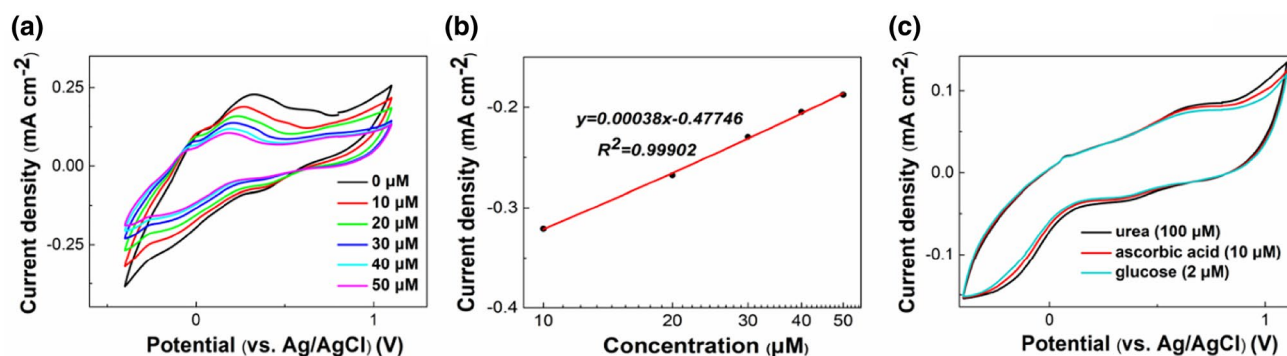
Fig. 7 a I - V responses of MWCNT/PANi-composite-modified SPCE at urea concentration range of 10–50 \mu\text{M} and scan rate of 50 \text{mV s}^{-1} . b Corresponding calibration curve. c I - V
