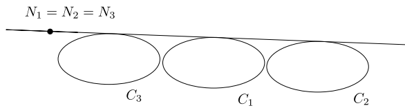
Fig. 3 Case 3 in Theorem 5.1
