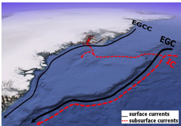
Fig. 5 Schematic of the major warm (red) and cold (black) currents over the Greenland shelf break and shelf including the East Greenland Current (EGC), East Greenland Coastal Current (EGCC) and Irminger Current (IC). The hypothesized trajectory of the Atlantic Water flowing from the shelf break through a canyon into the Sermilik Fjord is also shown
