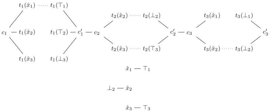
Fig. 5 The congruence graph for E_C \cup E_{\mathcal{I}}
