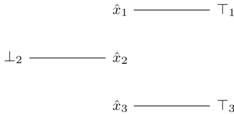
Fig. 2 The congruence translation E_C = Connect \cup \bigcup_{1 \leq i \leq n} Clause_i of \mathcal{C}
