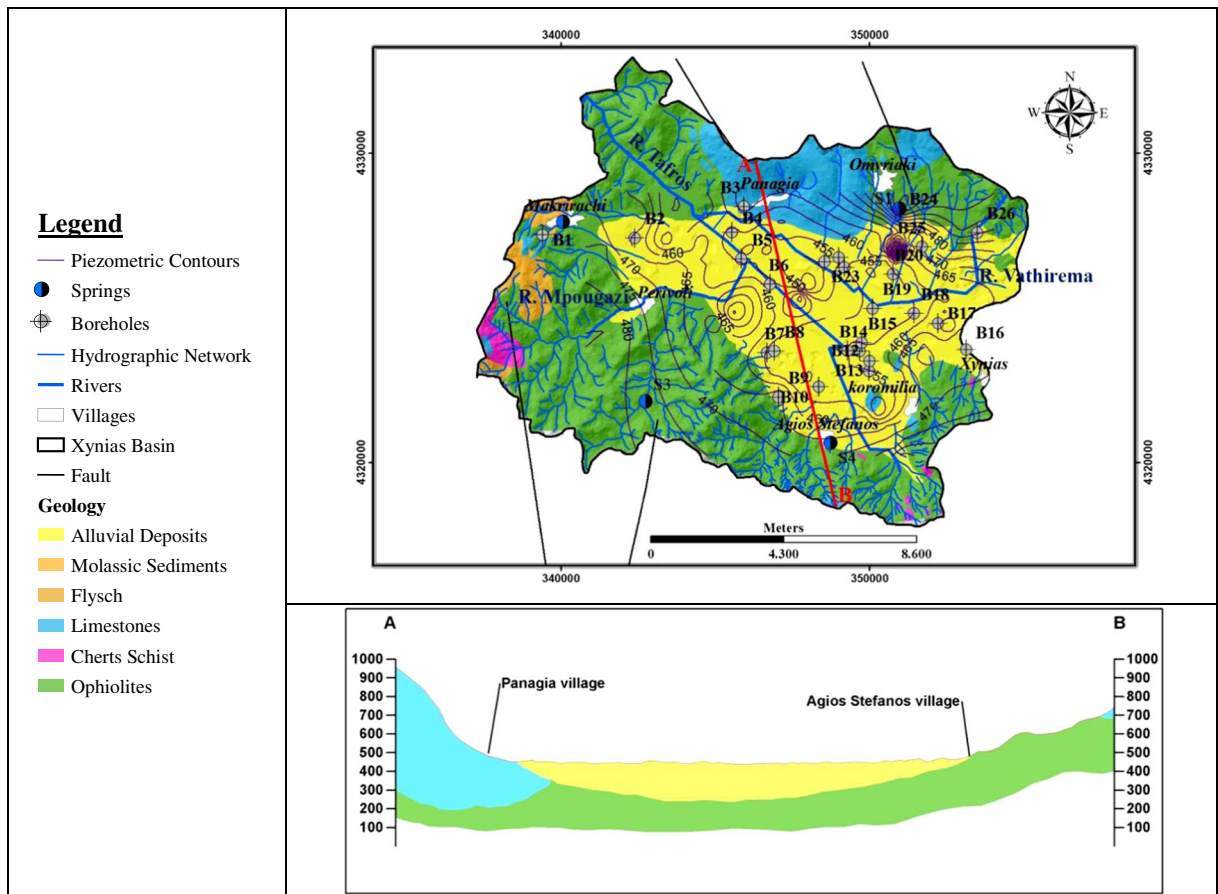
Fig. 2 Geology setting map and schematic geological cross section of the Xynias basin
