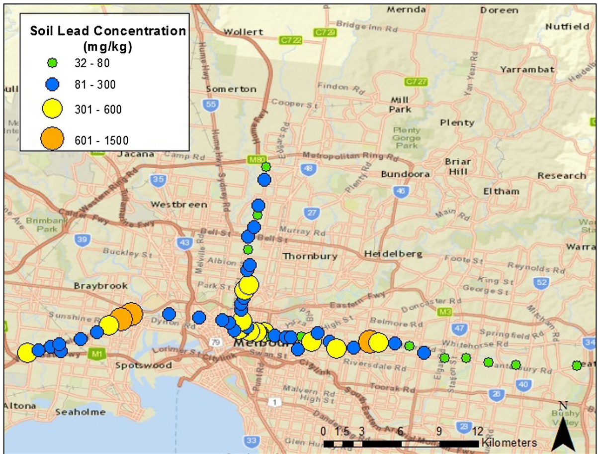
Fig. 1 Lead concentration (mg/kg) of surface soil (0–2 cm) samples collected along three transects oriented across the Melbourne metropolitan area (<250 \mu\text{m} grain size). Note Australian NEPC Residential HIL-A Soil Pb Guideline = 300 mg/kg (NEPC 2013a, b); Australian NEPC
