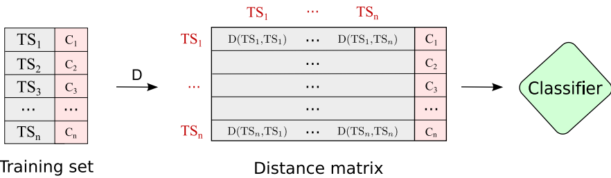
Fig. 3 A visual representation of the global distance features method
