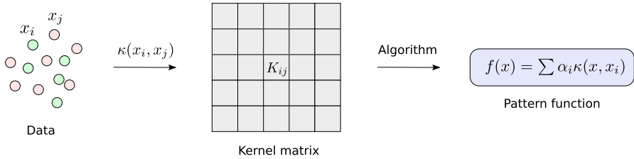
Fig. 7 The stages involved in the application of kernel methods (Shawe-Taylor and Cristianini 2004)
