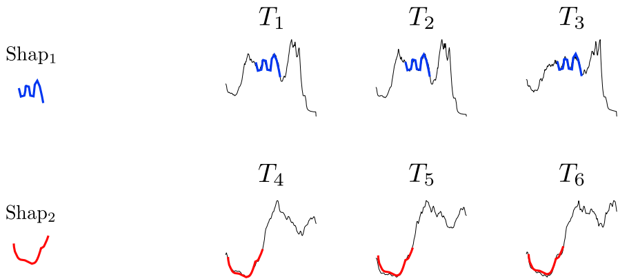
Fig. 4 Visual representation of two shapelets (Shap 1 and Shap 2 ) and six time series from the Coffee dataset (UCR). These shapelets are identified as being representative of class membership: Shap 1 belongs to class 1, as can be seen in the three time series (T 1 , T 2 and T 3 ) which belong to class 1, while Shap 2 belongs to class 2, as can be seen in the three time series (T 4 , T 5 and T 6 ) which belong to class 2
