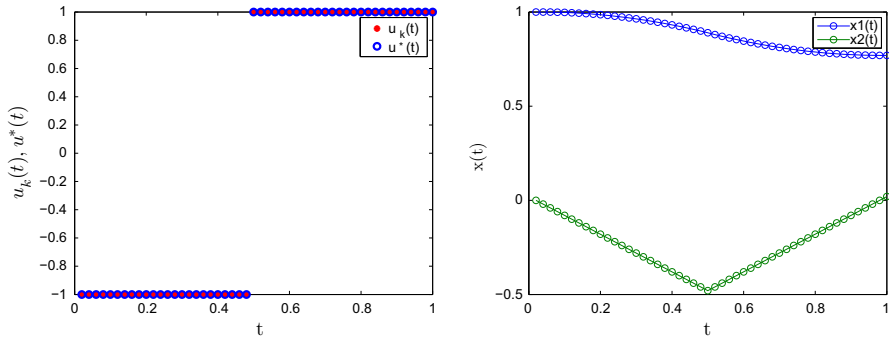
Fig. 1 Optimal control (left) and optimal states (right) for N = 50
