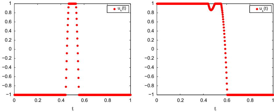
Fig. 3 Approximate optimal controls after 1000 iterations when \theta = 2 (left) and \theta = 3 (right) for Example 4.3 with N = 500
