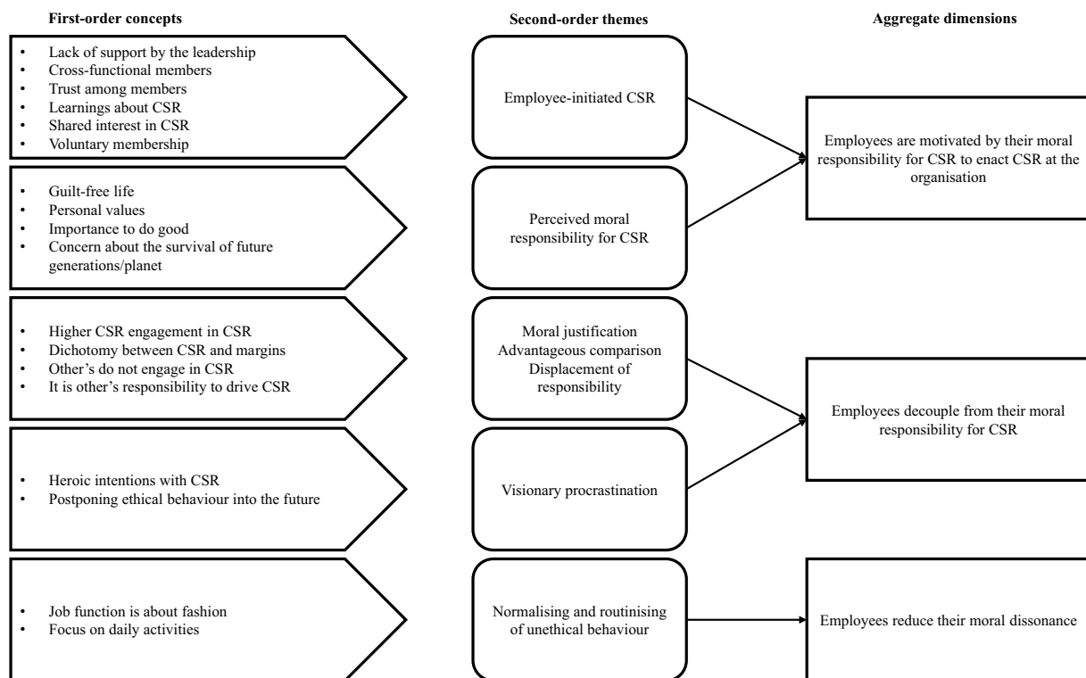
Fig. 1 Data structure
