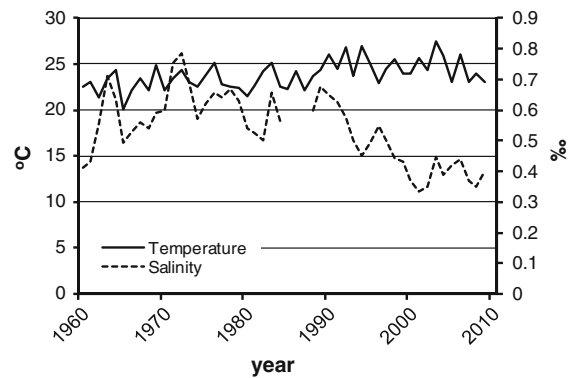
Fig. 3 Maximum water temperature and salinity of the river Rhine at Lobith (salinity measurements for the years 1985–1987 were not available)
