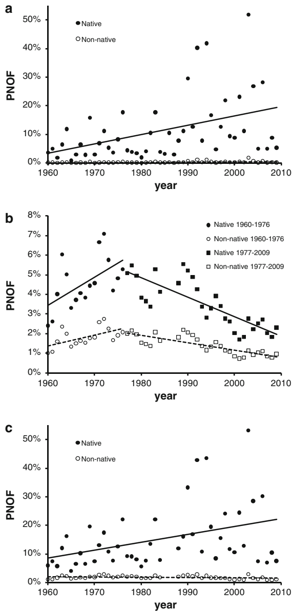
Fig. 4 Potentially not occurring fraction (PNOF) of native and non-native molluscs at Lobith in relation to yearly maximum water temperature conditions (a), yearly maximum salinity conditions (b) and both stressors combined under the assumption of additive effects (c) for the period 1960–2009
