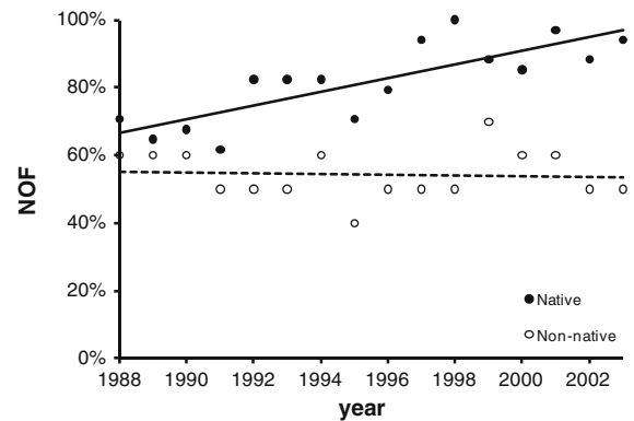
Fig. 5 Not occurring fraction (NOF) of native and non-native molluscs at Lobith derived from monitoring data for the period 1988–2003
