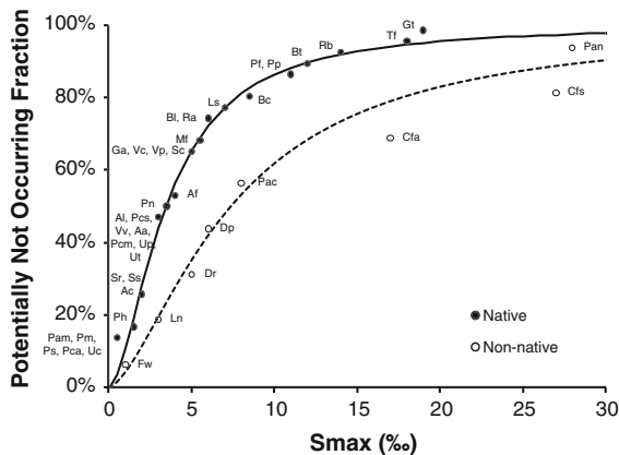
Fig. 2 Species sensitivity distributions for maximum salinity tolerances of native and non-native molluscs of the river Rhine. The data points represent individual species' tolerances based on Hazen plotting positions (Native: n = 33 ; \alpha = 0.54 , \beta = 0.25 ; Non-native: n = 8 ; \alpha = 0.87 , \beta = 0.27 ). Full species names can be found in Table 1
