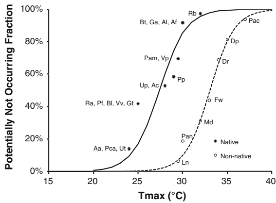
Fig. 1 Species sensitivity distributions for maximum temperature tolerances of native and non-native molluscs of the river Rhine. The data points represent individual species' tolerances based on Hazen plotting positions (Native: n = 18 ; \alpha = 27.39 , \beta = 1.49 ; Non-native: n = 8 ; \alpha = 33.06 , \beta = 1.39 ). Full species names can be found in Table 1
