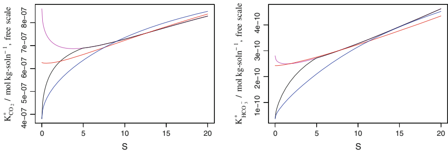
Fig. 1 Salinity dependence of four different S, t relationships of the first ( left panel ) and second ( right panel ) dissociation constant of the carbonate system. Magenta line Roy et al. (1993b), not adapted to low salinities (as implemented in seacarb ); red line Lueker et al. (2000), not valid below S = 19 (implemented in seacarb and AquaEnv ); black line Roy et al. (1993b), adapted to low salinities (as implemented in AquaEnv ); blue line Millero et al. (2006), valid down to S = 0 (implemented in AquaEnv )
