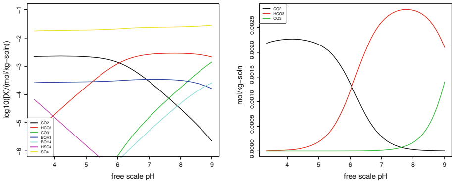
Fig. 7 Left panel Bjerrum plot of a selection of concentrations of dissociated species in the example in silico titration, concentrations are plotted on logarithmic scale. Right panel Bjerrum-like plot, concentrations are plotted on non-logarithmic scale
