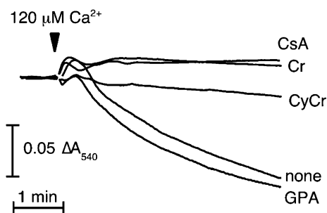
Fig. 4 Mitochondrial permeability transition is inhibited by CK substrates. At a concentration of 10 mM, the CK substrates creatine (Cr) and cyclocreatine (cCr), Cr-analogue, inhibit MPT in isolated mouse liver mitochondria to a comparable degree as 1 \mu M cyclosporin A (CSA), the gold standard for MPT inhibition (Dolder et al. 2003). The Cr-analogue guanidinopropionic acid (GPA) that is not accepted as a substrate by the CK reaction has no effect as compared to control without additions (none). Isolated liver mitochondria from transgenic mice expressing uMtCK in their liver were analysed by a swelling (light scattering) assay. They were energized with glutamate/malate in presence of 2mM Mg^{2+} and then challenged by 120 \mu M Ca^{2+} where indicated. (Figure taken from Dolder et al. 2003 with permission)
