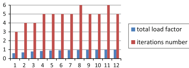
Fig. 3 Simple supported plate—number of iterations in the load incremental process
