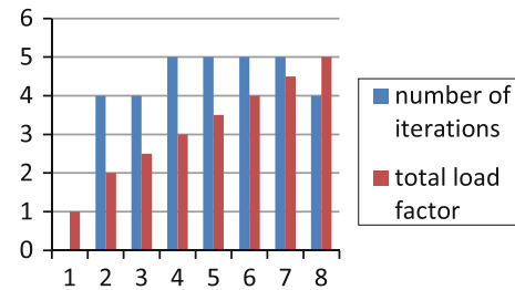
Fig. 10 Example 4—number of iterations in the load incremental process
