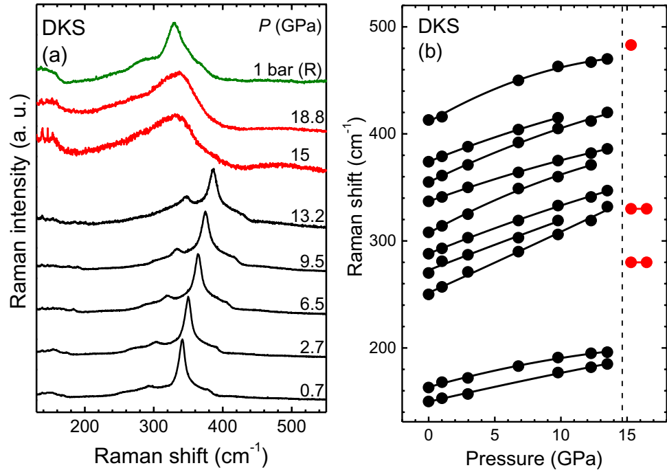
Fig. 4 a Raman spectra of Cu 2 ZnSnS 4 at selected pressures ( \lambda = 473 nm, T = 300 K). The black, red, and green spectra correspond to the DKS, GeSb-type, and ZB-type phases, respectively. b Raman mode frequency evolution as a function of pressure for the DKS (black) and the GeSb-type (red) Cu 2 ZnSnS 4 phases. The solid lines passing through the data points represent polynomial least square fittings. The vertical dashed line indicates the DKS-to-GeSb-type transition
