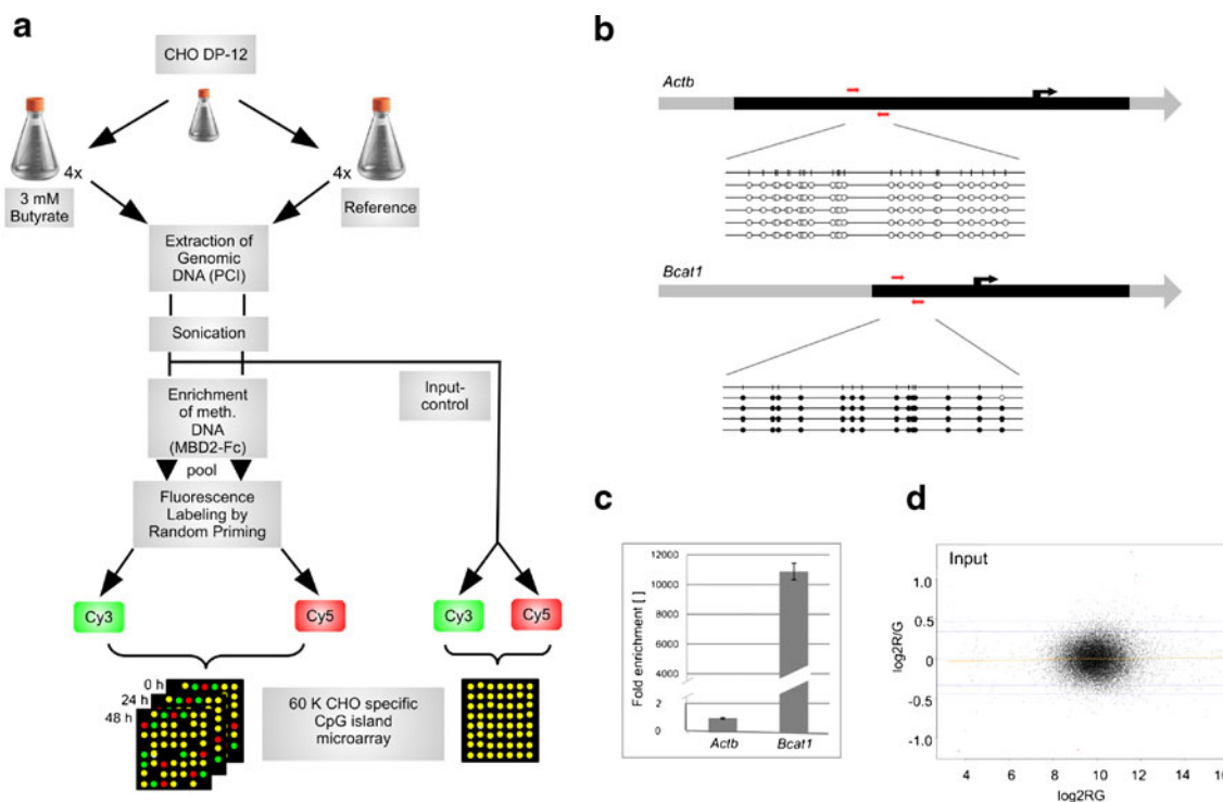
Fig. 1 Experimental design and quality control. a Schematic representation of methylated DNA enrichment combined with the CHO-specific CpG island microarray. b Bisulfite sequencing results of the CGIs of Actb and Bcat1 . The black region represents the CGI, the black arrow marks the transcription start site. Black circles represent a methylated CpG position, white circles indicate unmethylated CpG positions. The red
