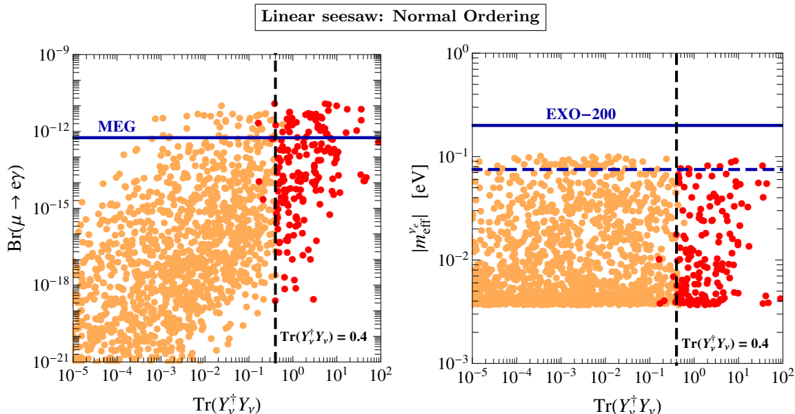
Figure 8. The same as in figure 6 but considering the linear seesaw.
