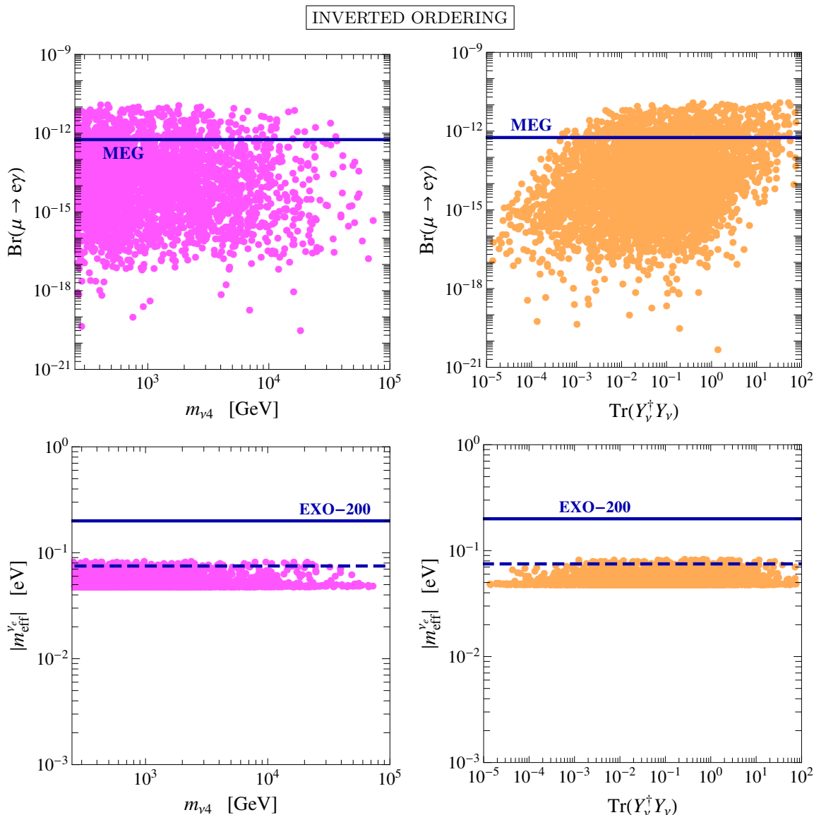
Figure 2. Same as in figure 1, but considering the inverted ordering.
