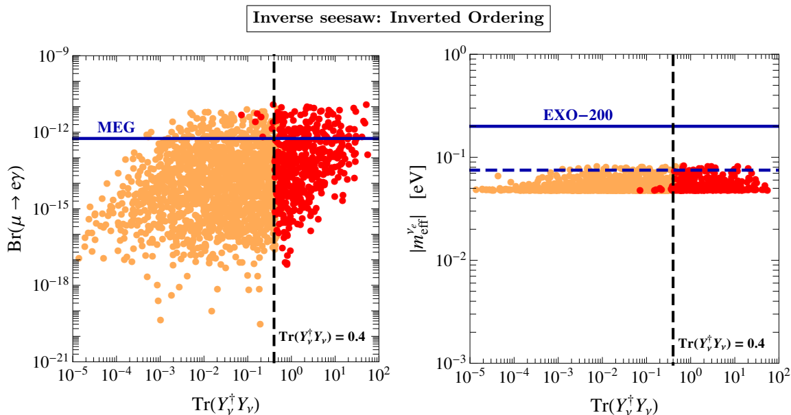
Figure 7. Same as in figure 6, but considering the inverted ordering.
