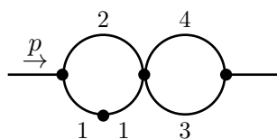
Figure 3. Double-bubble two-loop sub-topology.
