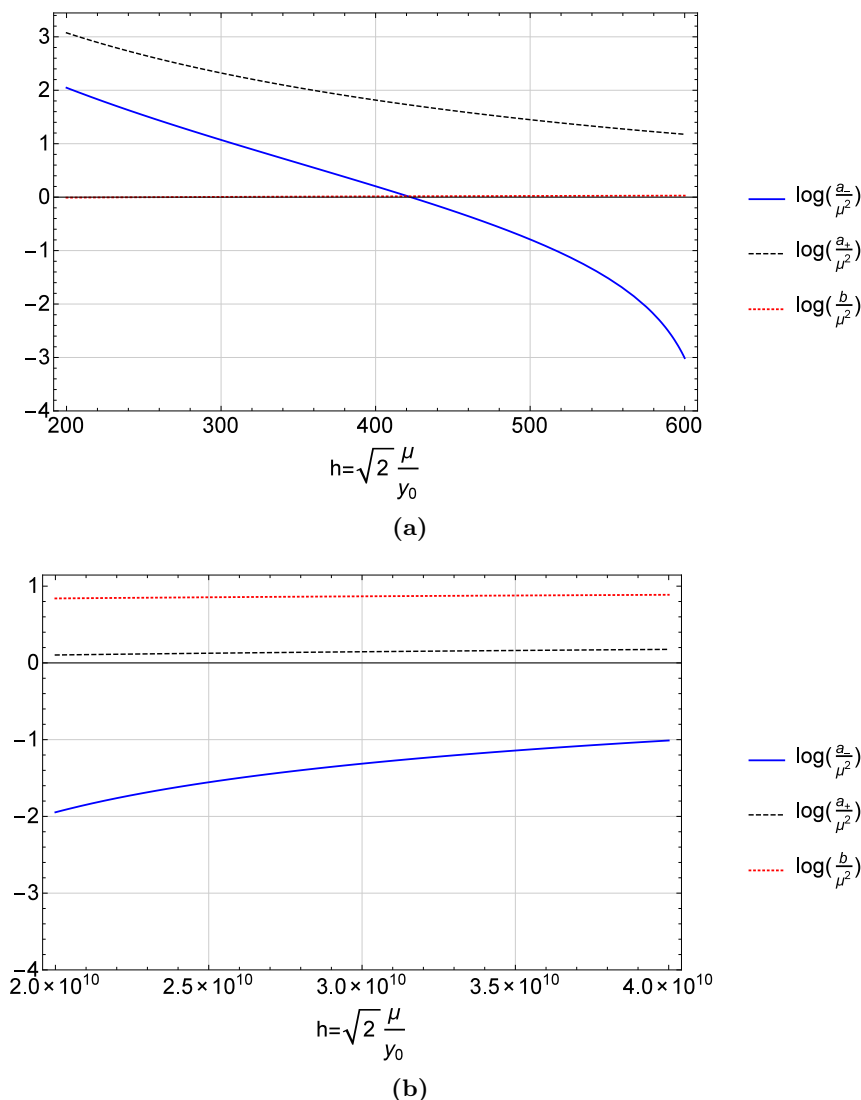
Figure 9. The logarithms of \{a_-, a_+, b\} for the chosen form of the running energy scale \mu = \frac{y_t}{\sqrt{2}}h .
