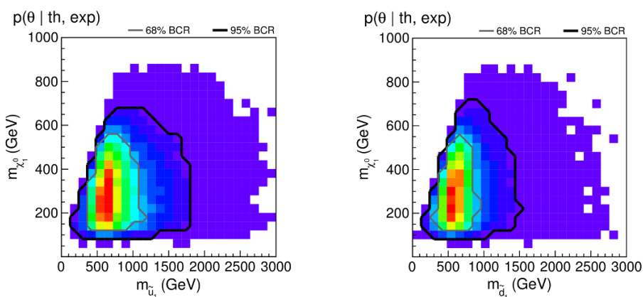
Figure 12. Correlations between the lightest neutralino mass and the lightest up- and down-type squark masses. Red colour indicates the highest likelihood.
