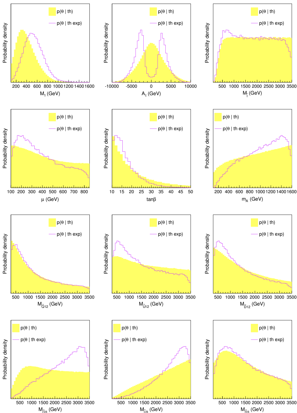
Figure 1. The one-dimensional prior (yellow histogram) and posterior (violet curve) distributions of the parameters of our NMFV MSSM description. The prior only incorporates theoretical inputs while the posterior distribution shows the impact of all experimental observations listed in table 3.
