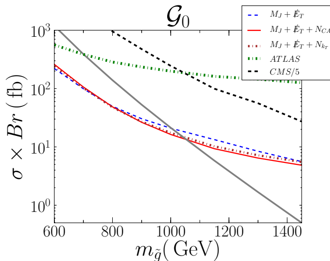
Figure 10. 95% exclusion limits on \sigma \times \mathcal{B} for the M_J + \cancel{E}_T search (dashed blue), the M_J + \cancel{E}_T + N_{CA} search (solid red), and the M_J + \cancel{E}_T + N_{k_T} search (dash-dotted brown) for signal \mathcal{G}_0 , which has only 4 final state partons. The exclusion limits given by the ATLAS high multiplicity search [56] (dash-dotted green line) and the CMS black hole search [57] (dashed black) as well as the NLO gluino production cross section (grey solid) are also shown. The systematic uncertainty on the background is assumed to be 30%. Note that the CMS limit is rescaled by a factor of 5.
