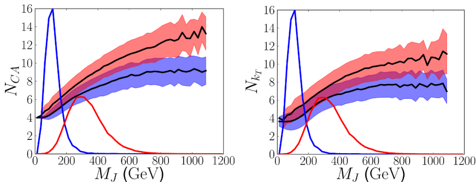
Figure 9. N_{CA} (left) and N_{kT} (right) versus M_J for signal topology \mathcal{G}_4 with m_{\tilde{g}} = 600 GeV (red band) and QCD background (blue band). Each band illustrates \pm 1\sigma standard deviation about the mean, which is denoted by a black line. The superimposed M_J distributions are for the signal (red) and the QCD background (blue). As defined in Sec 2, N_{CA} and N_{kT} are the sum of the number of subjets of the four leading jets of each event. The events considered are required to have at least four jets with p_T > 50 GeV and the p_T of their leading jet must be greater than 100 GeV.
