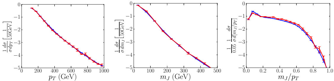
Figure 4. Comparison between SHERPA (red) and MadGraph+PYTHIA (blue) for three relevant kinematic variables of the leading jet.
