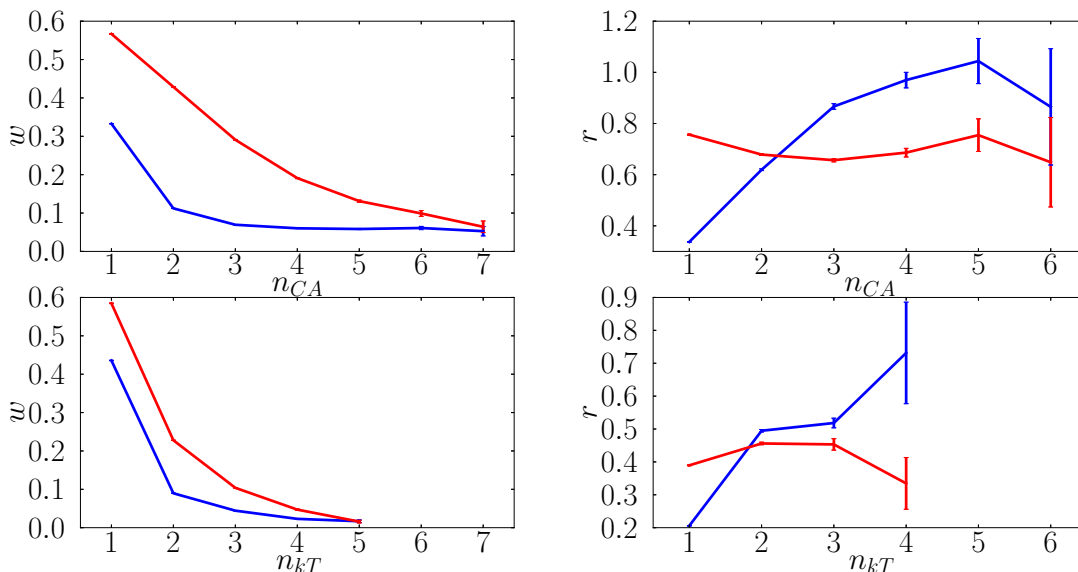
Figure 3. Scaling patterns for the subjet distributions of leading QCD fat jets generated by MadGraph. Left: the ratio w(n) for n_{k_T} (bottom) and n_{CA} (top) for jets with p_T \geq 100 GeV (blue) and p_T \geq 500 GeV (red). “Staircase scaling” corresponds to a flat w(n) . Right: the ratio r(n) for n_{k_T} (bottom) and n_{CA} (top) for jets with p_T \geq 100 GeV (blue) and p_T \geq 500 GeV (red). “Double staircase scaling” corresponds to a flat r(n) and appears to be emerging in the high p_T regime.
