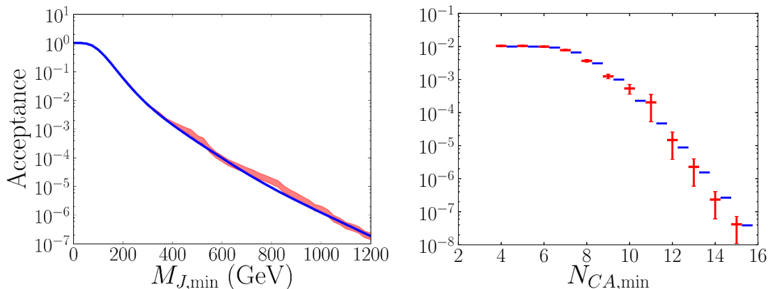
Figure 7. Testing the jet template ansatz. The figure on the left compares the raw M_J cut acceptance (red) to the template estimate (blue). The figure on the right is analogous, with a sliding N_{CA} cut and a fixed cut M_J > 280 GeV. The red uncertainties are statistical (the statistical uncertainties for the template estimate are not shown, since by construction they are parametrically smaller than the raw uncertainties).
