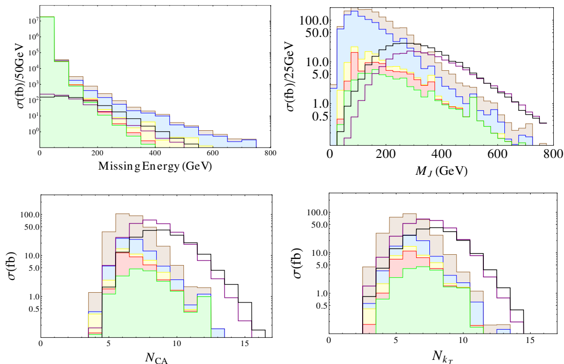
Figure 8. Top left: \cancel{E}_T distributions for signals and backgrounds after requiring four or more fat jets. Top right: M_J distributions, after requiring four or more fat jets and \cancel{E}_T > 150 GeV. Bottom left: N_{CA} distribution after requiring four or more fat jets, M_J > 280 GeV and \cancel{E}_T > 150 GeV. Bottom right: N_{kT} distribution after requiring four or more fat jets, M_J > 280 GeV and \cancel{E}_T > 150 GeV. Stacked histograms show the SM backgrounds, which include top and single top (light brown), V + nj (light blue), diboson (light yellow), QCD (light green), and the remaining non-QCD backgrounds mentioned in Sec 3.1 (light red). The distributions for a 600 GeV gluino in the \mathcal{G}_1 and \mathcal{G}_3 topologies are shown in purple and black, respectively. Note that the N_{CA} and N_{kT} distributions for \mathcal{G}_3 (with 20 final state partons) are not substantially different from \mathcal{G}_1 (with 12).
