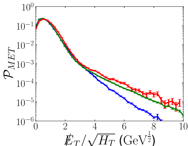
Figure 6. The missing energy significance, y = \cancel{E}_T/\sqrt{H_T} ( \text{GeV}^{\frac{1}{2}} ) in three different H_T bins: [300, 600] GeV (blue), [900, 1200] GeV (green), and [1500, 1800] GeV (red).
