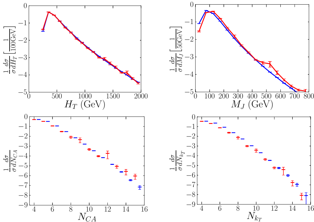
Figure 5. Comparison between SHERPA (red) and MadGraph+PYTHIA (blue) for H_T (upper left), M_J (upper right), N_{CA} (lower left) and N_{k_T} (lower right). For the definition of the latter two observables see section 2. For the bottom two distributions, the MadGraph+PYTHIA points have been shifted by half a unit to the right in order to facilitate the comparison.
