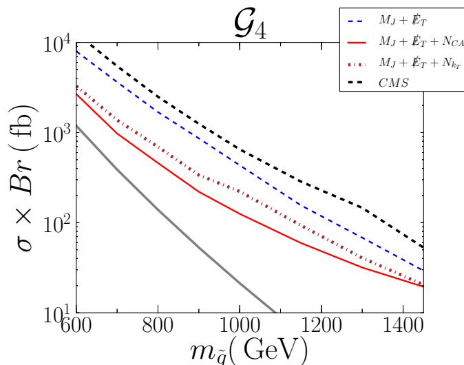
Figure 11. 95% exclusion limits on \sigma \times \mathcal{B} for the M_J + \cancel{E}_T search (dashed blue), the M_J + \cancel{E}_T + N_{CA} search (solid red), and for the M_J + \cancel{E}_T + N_{k_T} search (dash-dotted brown) for signal \mathcal{G}_4 , which has 10 final state partons and no intrinsic \cancel{E}_T . The exclusion limit given by the CMS black hole search [57] (dashed black) as well as the NLO gluino production cross section (grey solid line) are also shown. The systematic uncertainty on the background is assumed to be 30%. The ATLAS limit is not shown because it is orders of magnitude worse than the others due to its strict \cancel{E}_T requirement.
