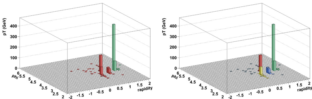
Figure 1. Example of a fat (and very massive) QCD jet with p_T = 910 GeV, m = 360 GeV and with its two n_{k_T} subjets (left) and its four n_{CA} subjets (right) indicated. Note that this jet has not been trimmed to better illustrate the different treatment of soft radiation in n_{CA} and n_{k_T} (the dark gray cells on the right do not belong to any identified subjets).
