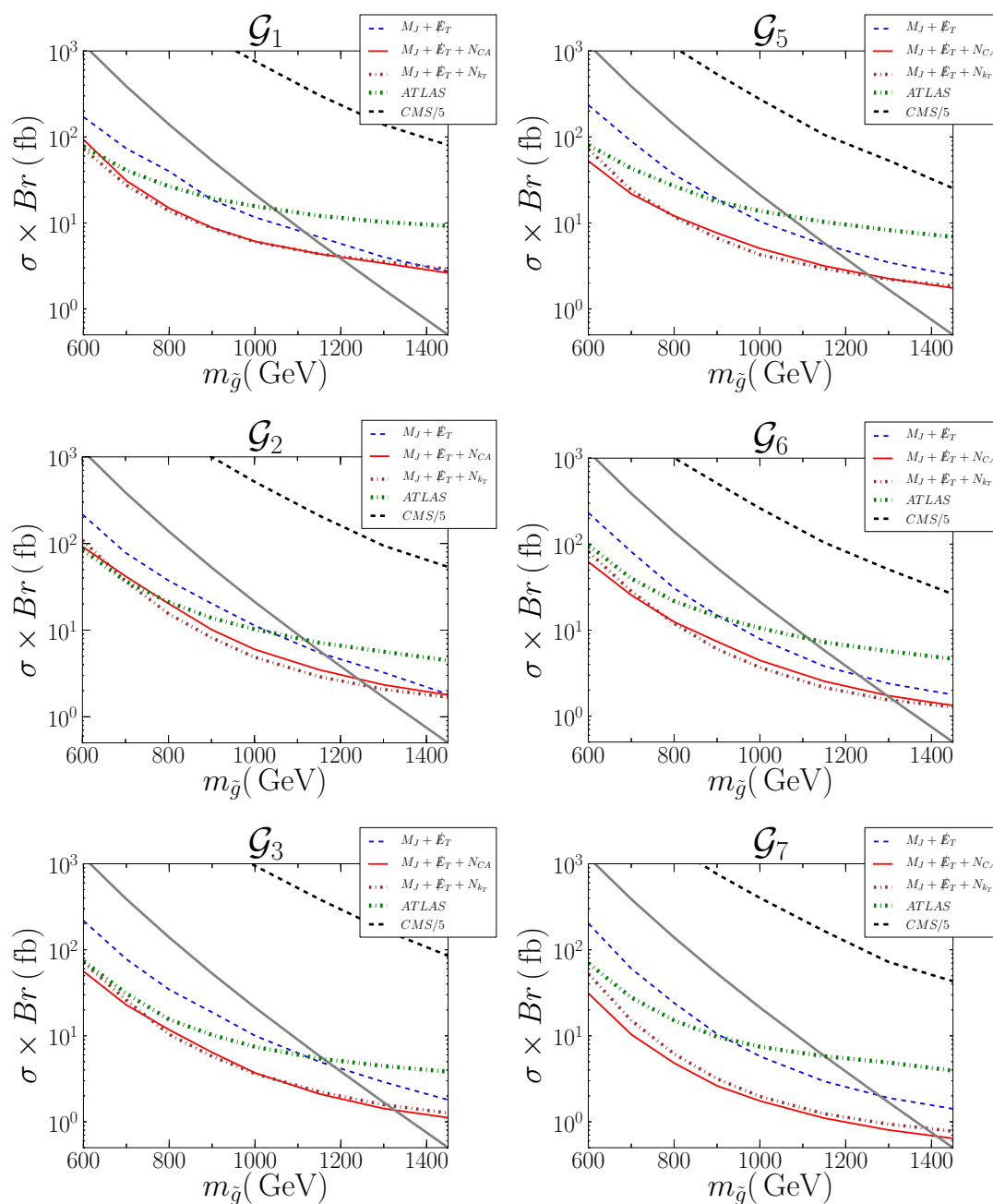
Figure 12. 95% exclusion limits on \sigma \times \mathcal{B} for the M_J + \cancel{E}_T search (dashed blue), the M_J + \cancel{E}_T + N_{CA} search (solid red), and the M_J + \cancel{E}_T + N_{kr} search (dash-dotted brown) for the R-parity conserving topologies \mathcal{G}_1 , \mathcal{G}_2 , and \mathcal{G}_3 (left, top to bottom) and the corresponding RPV ones, \mathcal{G}_5 , \mathcal{G}_6 , and \mathcal{G}_7 (right, top to bottom). The exclusion limits given by the ATLAS high multiplicity search [56] (dash-dotted green) and the CMS black hole search [57] (dashed black) as well as the NLO gluino production cross section (grey solid line) are also shown. The systematic uncertainty on the background is assumed to be 30%. Note that the CMS limit is rescaled by a factor of 5.
