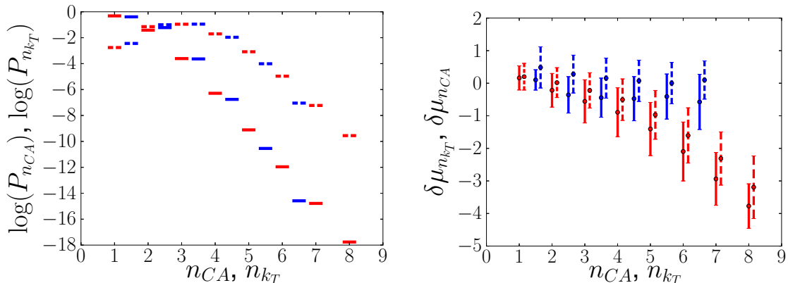
Figure 2. Left: The subject distributions \log_{10} P_{n_{k_T}}(n_{k_T}) and \log_{10} P_{n_{CA}}(n_{CA}) in blue and red, respectively. Right: The blue and red distributions show \delta\mu_{n_{CA}}(n_{k_T}) and \delta\mu_{n_{k_T}}(n_{CA}) , respectively, which are defined in eq. (2.7). The error bars on \delta\mu_{n_{CA}}(n_{k_T}) and \delta\mu_{n_{k_T}}(n_{CA}) correspond to the standard deviations \sigma_{n_{CA}} and \sigma_{n_{k_T}} . For both panels the solid lines correspond to a sample of leading QCD jets generated by MadGraph and with p_T \geq 100 GeV, while dashed lines correspond to a signal-like sample described in the text.
