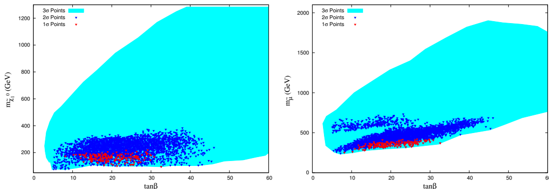
Figure 6. Correlations between low scale parameters: (Left panel) lightest neutralino mass ( m_{\tilde{\chi}_1^0} ) vs \tan\beta ; (Right panel) smuon mass ( m_{\tilde{\mu}} ) vs \tan\beta , depending on [1 \div 3]\sigma muon ( g-2 ) excess after satisfying all other constraints discussed in the text. A very similar correlation in m_{\tilde{\nu}} - \tan\beta plane is found as given in plot on the Right Panel. The slepton and sneutrino mass difference varies from 5-20 GeV, indicating that the sneutrino-wino loop in figure 3 may also contribute significantly.
