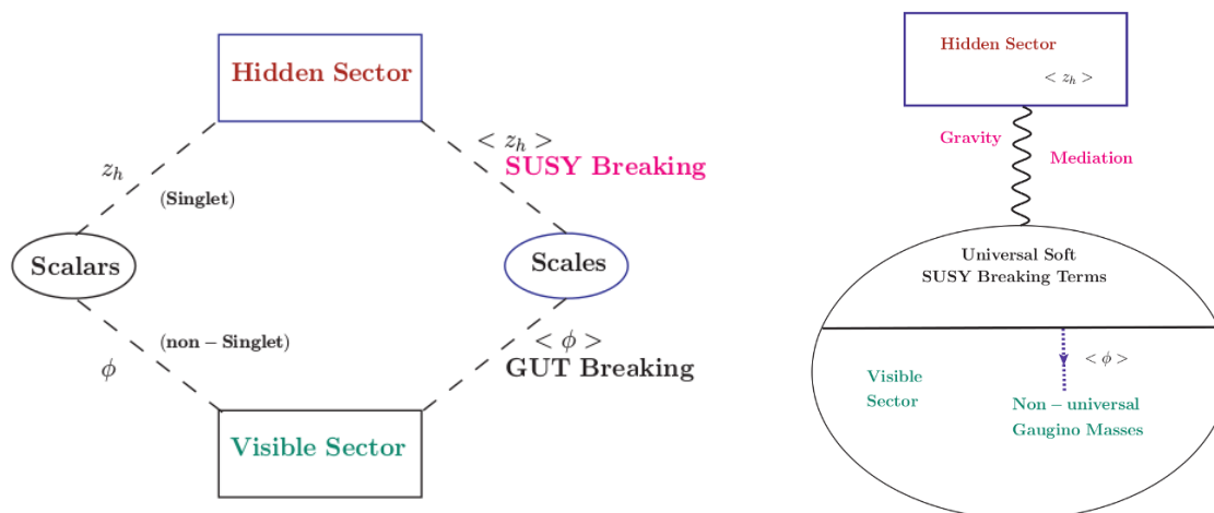
Figure 1. Schematic flow chart to demonstrate spontaneous breaking of supersymmetry in the hidden sector through the VEV of the singlet chiral super-field ( z_h ) and successive breaking of GUT symmetry in the visible sector through the VEV of non-singlet chiral super-field ( \phi ). As the outcome of this process, the soft SUSY breaking terms are generated in the visible sector and the gauginos become non-degenerate at the high scale itself.
