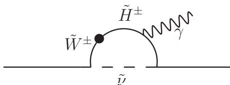
Figure 3. Feynman diagrams that contribute to muon (g-2) involving charginos ( \tilde{W}^\pm, \tilde{H}^\pm ) and sneutrino ( \tilde{\nu} ).
