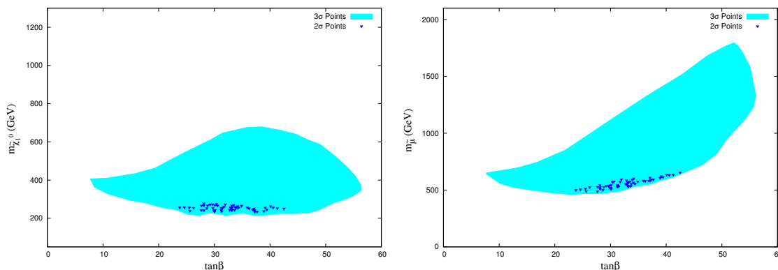
Figure 10. Correlations between low scale parameters: (Left panel) lightest neutralino mass ( m_{\tilde{\chi}_1^0} ) vs \tan\beta ; (Right panel) smuon mass ( m_{\tilde{\mu}} ) vs \tan\beta , depending on [2 \div 3]\sigma muon (g-2) excess after satisfying all other constraints discussed in the text. A very similar correlation in m_{\tilde{\nu}}-\tan\beta plane is found as given in plot on the Right Panel. We have not found any parameter space in this scenario that satisfy 1\sigma excess.
