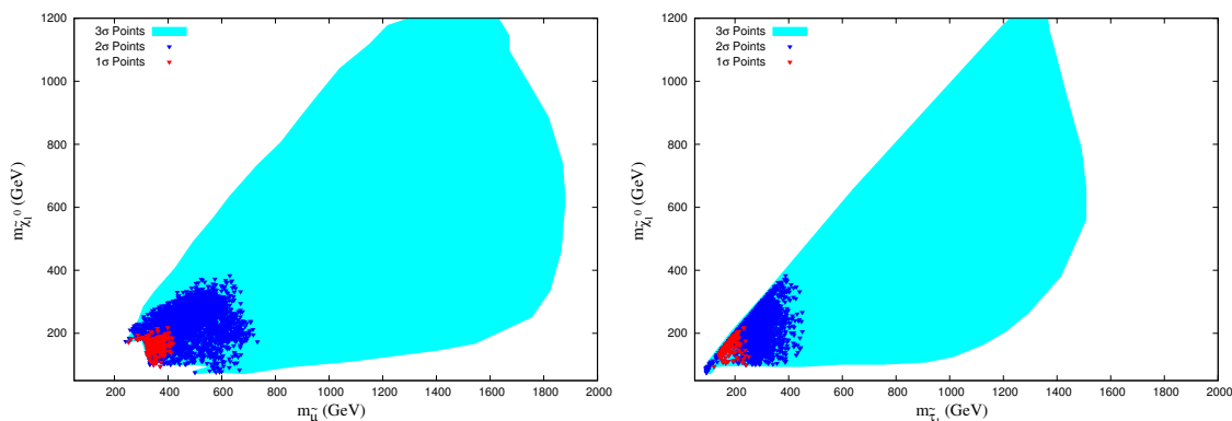
Figure 7. Correlations between low scale parameters: (Left panel) lightest neutralino mass ( m_{\tilde{\chi}_1^0} ) vs smuon mass ( m_{\tilde{\mu}} ); (Right panel) lightest neutralino mass vs stau mass ( m_{\tilde{\tau}_1} ), depending on [1 \div 3]\sigma muon (g-2) excess after satisfying all other constraints discussed in the text.
