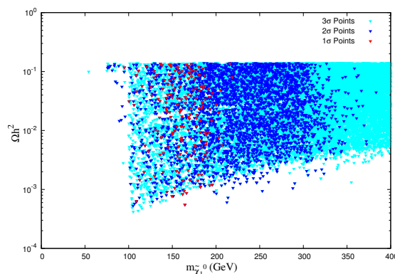
Figure 8. Relic density as a function of the mass of the dark matter, i.e., LSP ( \tilde{\chi}_1^0 ) depending on [1 \div 3]\sigma muon (g-2) excess after satisfying all other constraints discussed in the text.
