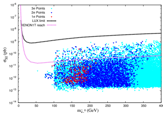
Figure 9. Direct detection cross-section as a function of the mass of the dark matter, i.e., LSP ( \tilde{\chi}_1^0 ) depending on [1 \div 3]\sigma muon (g-2) excess after satisfying all other constraints discussed in the text.
