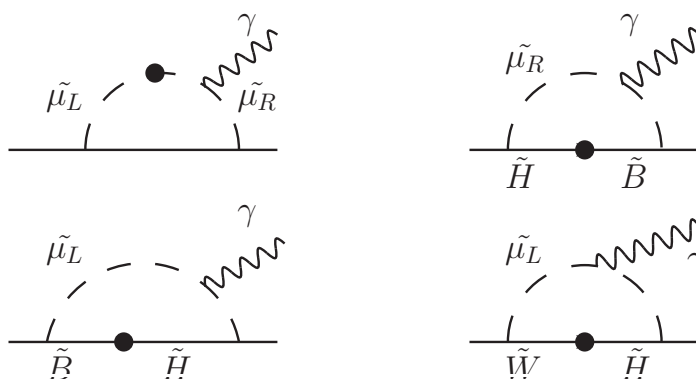
Figure 2. Feynman diagrams that contribute to muon ( g-2 ) involving neutralinos ( \tilde{B}, \tilde{W}, \tilde{H} ) and smuons ( \tilde{\mu}_{L,R} ).
