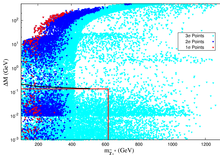
Figure 4. Impact of constraints from search for disappearing track and long lived particles, see section 4.1. The region enclosed by the red lines is excluded from long-lived or stable charged particle search. The area under the slanted black line just above the horizontal red line is excluded from disappearing charged track search at the LHC.
