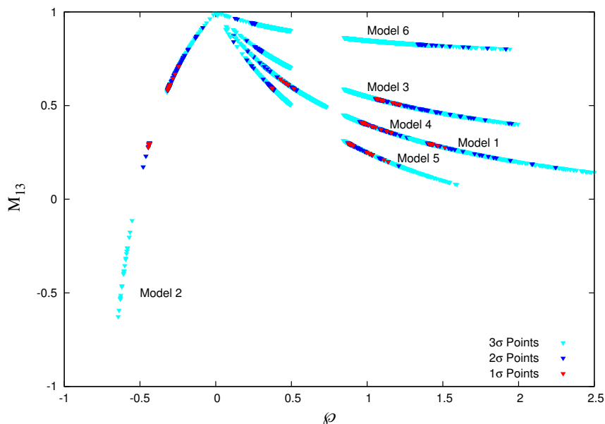
Figure 11. The variations of mixing parameter \varphi with M_{13} for different set of models leading to [1 \div 3]\sigma excess in muon (g-2). The other models cannot provide \Delta a_\mu excess at level of [1 \div 2]\sigma .
