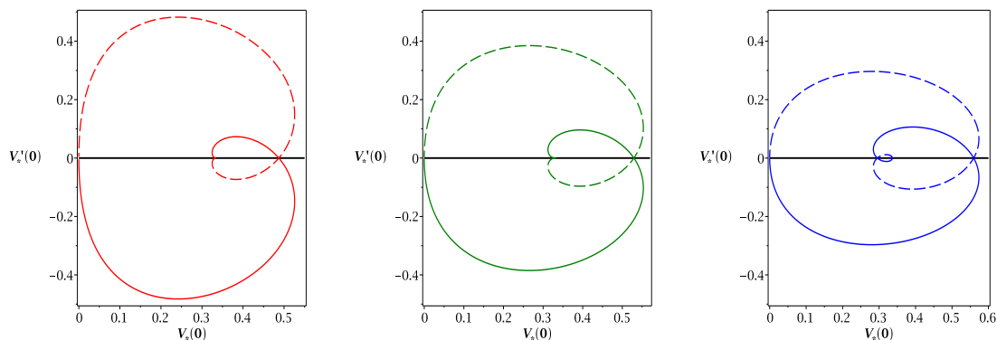
Figure 4. Varying the asymptotic parameter A from A = 0 to A \rightarrow \infty , for different values of \alpha leads to these spirals in V_*(0), V'_*(0) - space, where A = 0 corresponds to the point (V'_*(0) = 0, V_*(0) = 1/3) , and A \rightarrow \infty tends to the origin. From left to right the curves show \alpha = 0.5 (red), \alpha = 1 (green) and \alpha = 2 (blue). The dashed curves correspond to the solid curves reflected in the V_*(0) axis. From the discussion below (2.14), we know that fixed point solutions correspond to the points where the solid and dashed curves cross.
