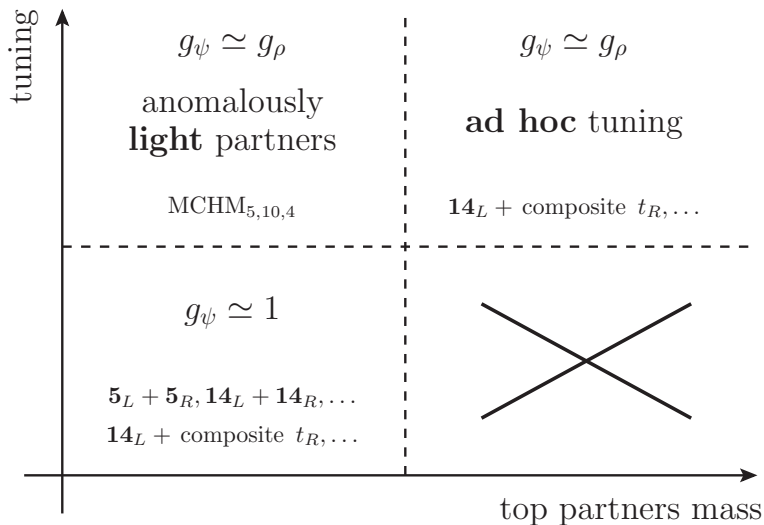
Figure 8. Schematic representation of the properties of the three basic classes of composite-Higgs models.
