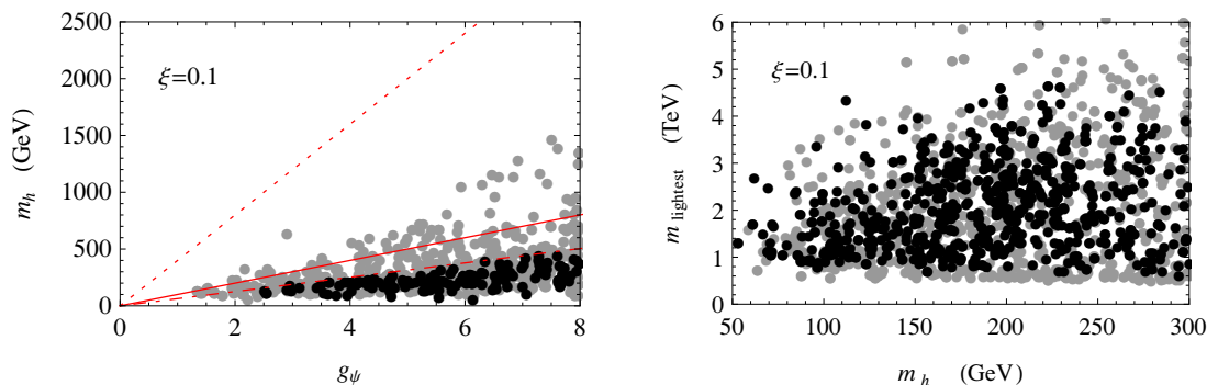
Figure 5. Scatter plots in the \text{CHM}_{14} set-up with composite t_R for \xi = 0.1 in the region of nearly degenerate 9 and 4 (we allow for a maximal 10% split in the mass parameters). In the left panel we show the Higgs mass as a function of g_\psi and in the right panel the mass of the lightest fermionic resonance as a function of the Higgs mass. For the colors of the points and the meaning of the red lines see the caption of figure 4.
