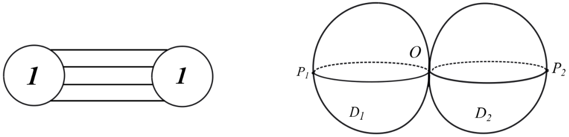
Figure 1. Left: the affine A_1 Dynkin diagram. Right: the nilpotent cone of Hitchin fibration for \widetilde{\mathcal{M}}_{2,1} , consisting of two \mathbb{CP}^1 intersecting at O with intersection number 2. Together with P_1, P_2 , they comprise the three fixed points of the Hitchin moduli space \widetilde{\mathcal{M}}_{2,1} .
