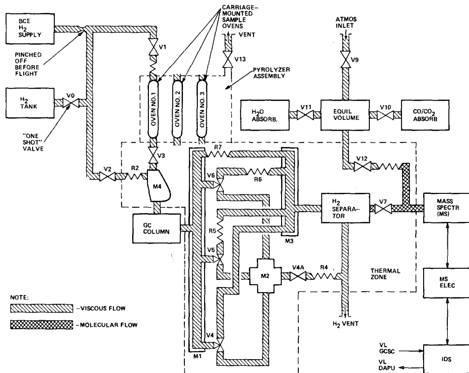
Fig. 1. Gas Flow Block Diagram. Dotted line delineates the heated zone (4 in Figure 2). M1, M2, V4-6 and R4-7 represent the effluent divider (see text).
