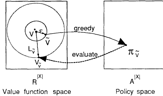
Figure 1. Loss from approximate optimal-value functions. Given \tilde{V} , an approximation within \epsilon > 0 of V^* , derive the corresponding greedy policy \pi_{\tilde{V}} . The resulting loss in value, V^* - V_{\tilde{V}} , is bounded above by (2\gamma\epsilon)/(1 - \gamma) .
