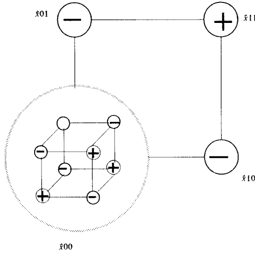
Figure 2. Examples used to show that 2-CASCADE NEURAL NET TRAINING is \mathfrak{U}\mathcal{P} -complete.
