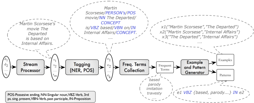
Fig. 2. Workflow of Processes for Discovering Examples
