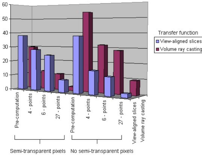
Fig. 3. Data from Table 1 presented in the chart. Depends of average performance speed (fps) of 3D models as a function of rendering algorithm type, gradient computation method and transfer function.
