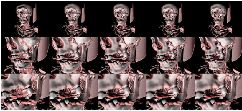
Fig. 4. Volume rendering of example model with different methods of gradient estimation. From left to right: intermediate difference, central difference, Sobel, Neumann and Zucker-Hummel.
