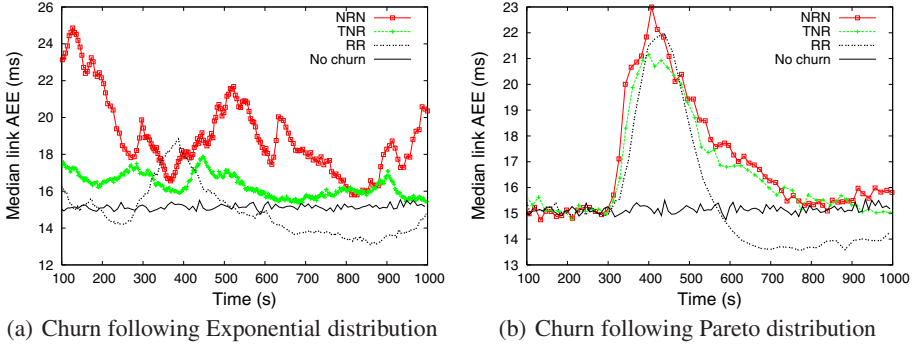
Fig. 6. Meridian dataset: Median absolute error as function of time
