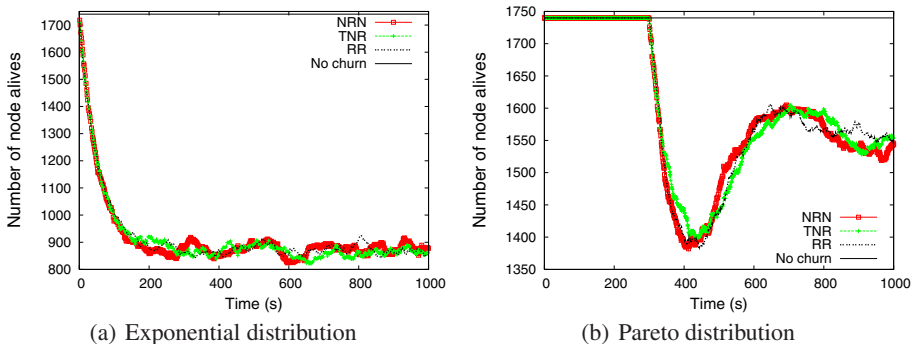
Fig. 1. King dataset: nodes alive as function of time
