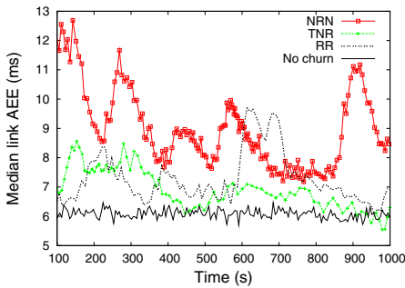
(a) Churn following Exponential distribution
