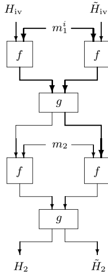
Fig. 3. The collision attack. Thick lines mean that there are r different values of this variable. Thin lines mean that there is only one.
