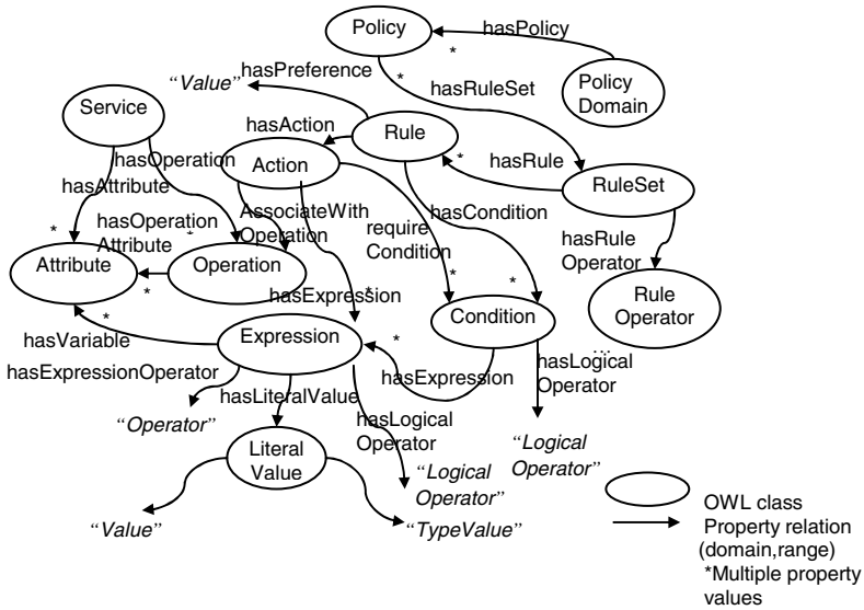
Fig. 2. Upper ontology for business rules policy
