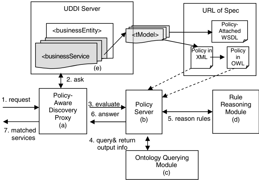
Fig. 5. Policy-based discovery framework
