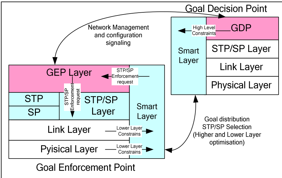
Fig. 3. GBN and STP/SP reference Model
