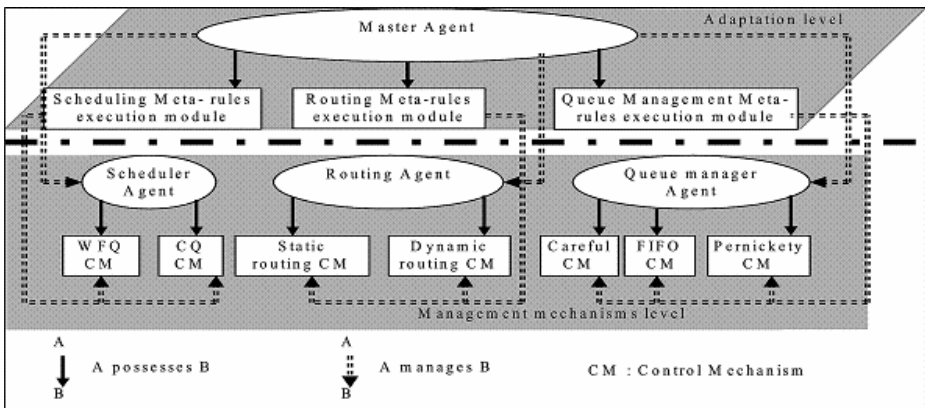
Fig. 1. Two levels of decision within the node
