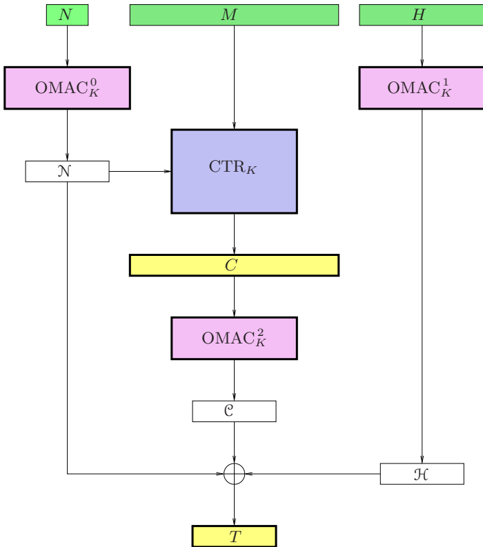
Fig. 3. Encryption under EAX. The message is M , the key is K , and the header is H . The ciphertext is CT = C \parallel T
